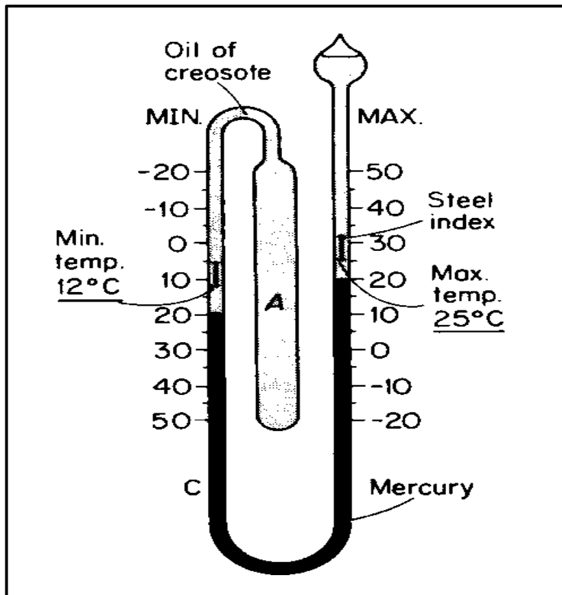
Six's thermometer
